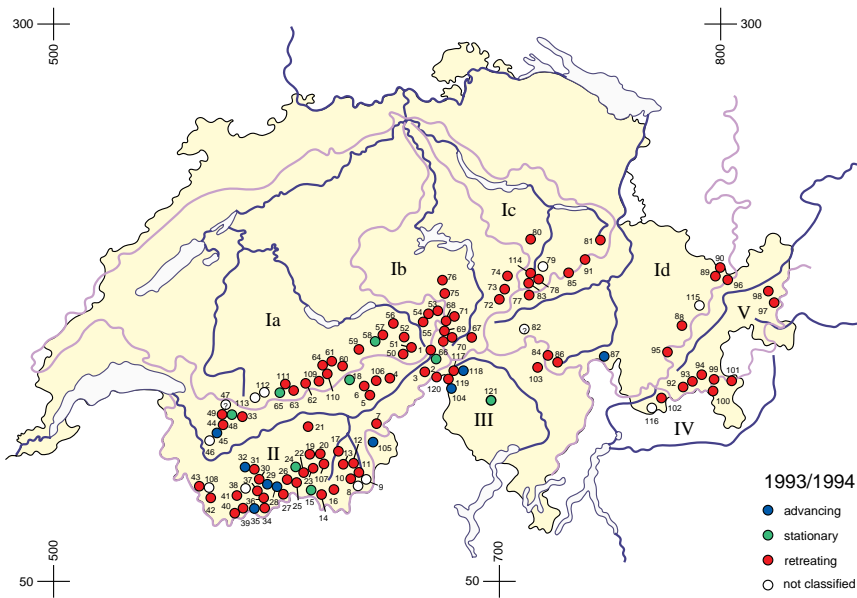
Figure 2.3a: Observed glaciers 1994.
