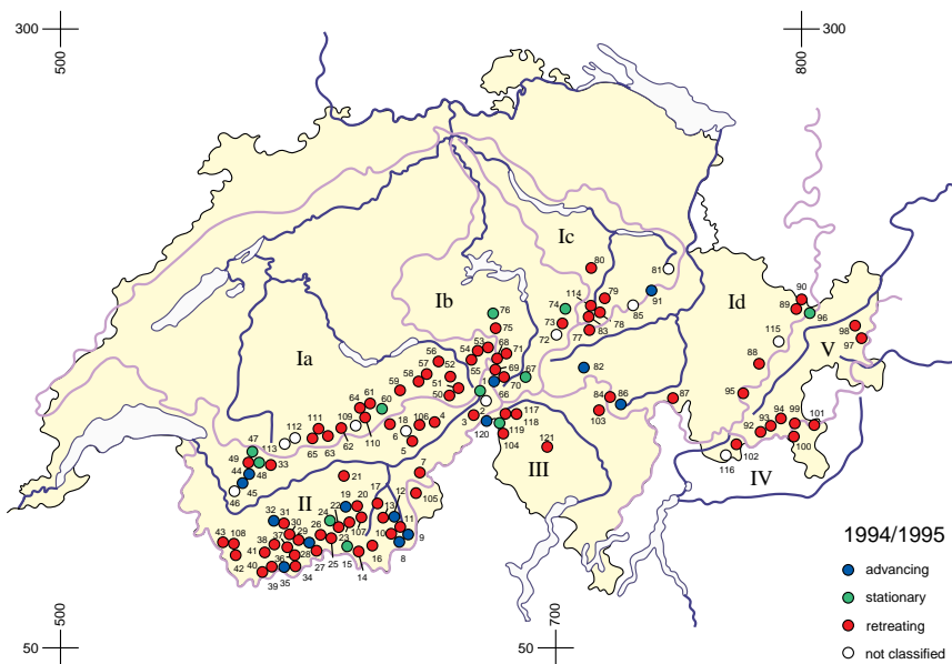
Figure 2.3b: Observed glaciers 1995.
