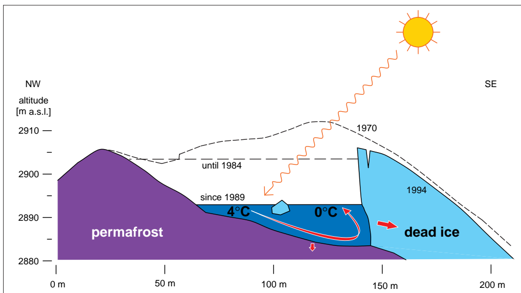
Figure 6.1: The process operating in Lake 5: Between the dead ice (right) and the permafrost a crack formed which filled with water. Lake water warms up by the sun and drops because of the density increase. At the dead ice it cools down again and then rises. This initiates water circulation which increases the volume of Lake 5 continuously. This lake also threatened to burst out and was, therefore, evacuated.
